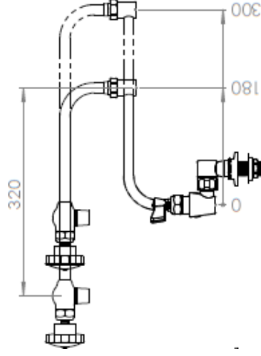
DOUBLE SWIVEL View
