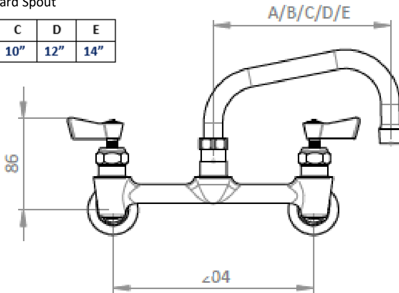
Standard Spout
