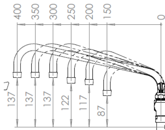
SIDE VIEW STANDARD SPOUT
